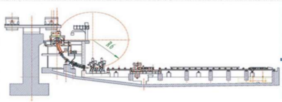
R6m 全弧标准型连铸机 Standard type R6m all arc continuous casting machine
