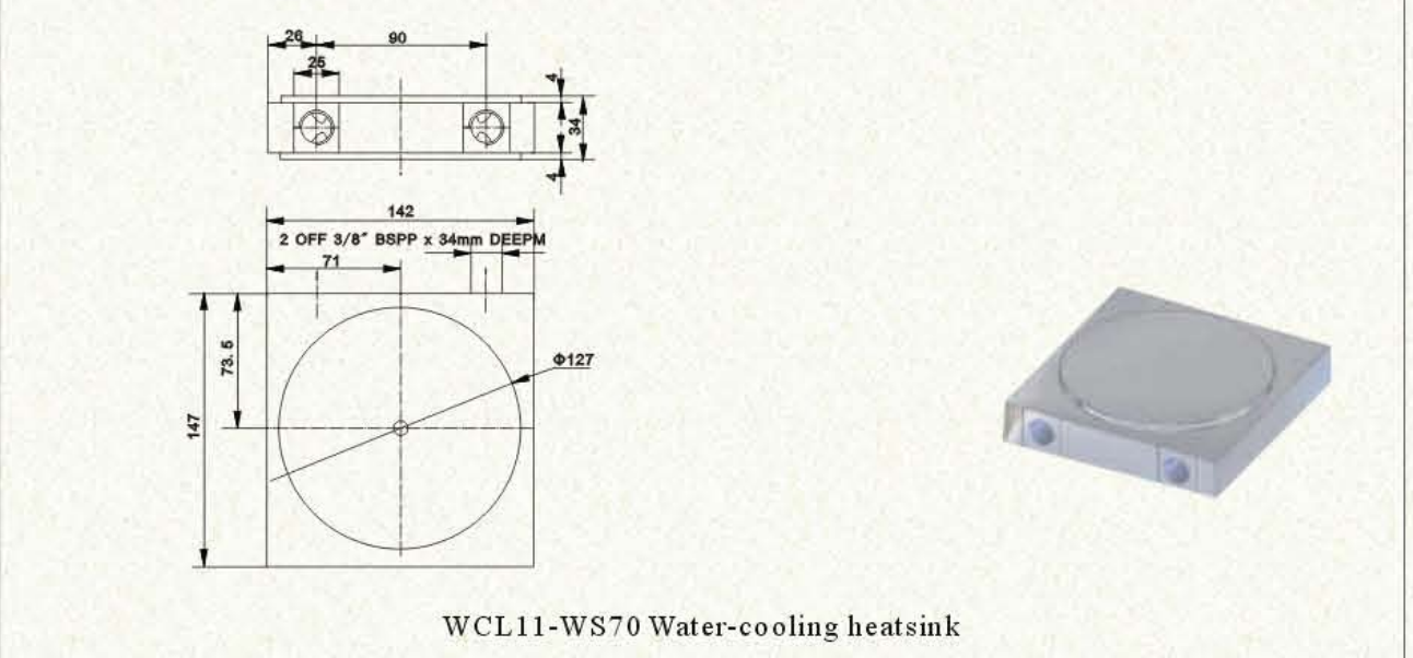
XW127EC25B Water-cooling heatsink
