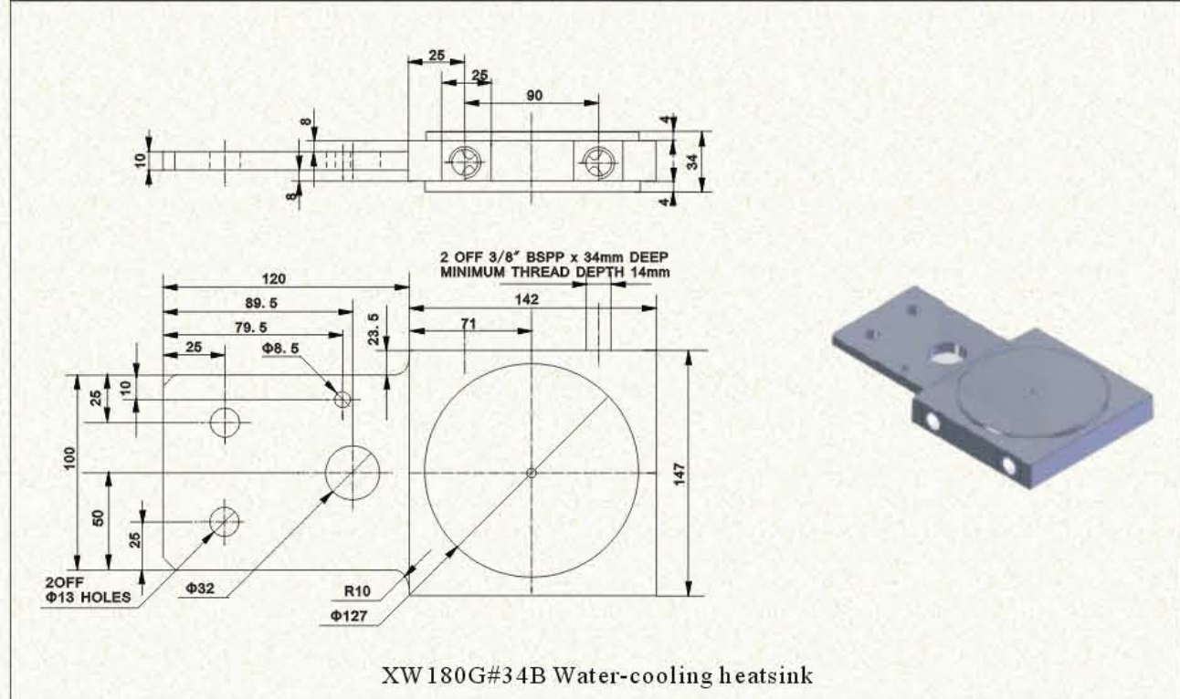
WCL14-WS72-1 Water-cooling heatsink
